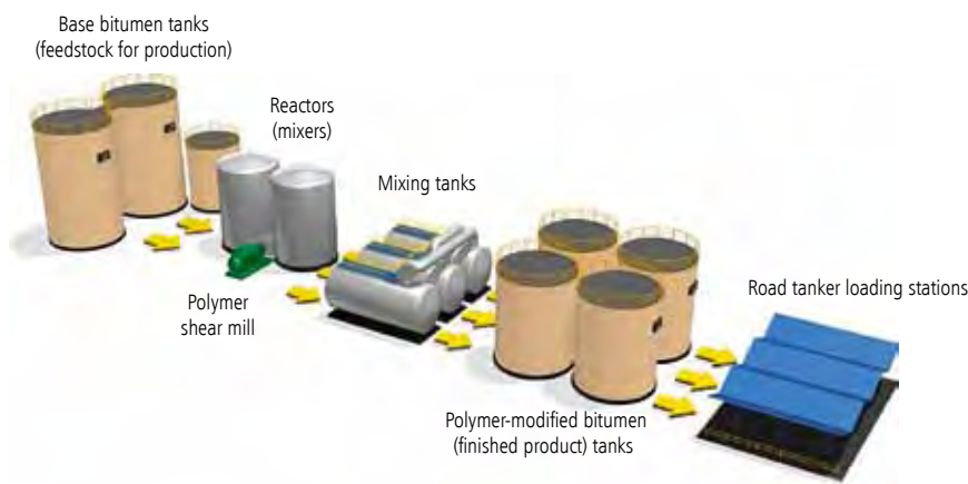
Figure 1.3. Płock site bitumen modification system diagram
