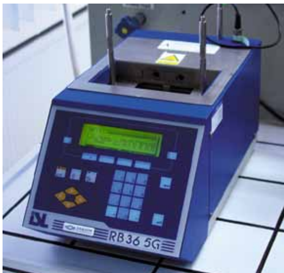
Figure 2.5. General view of the automatic R&B softening point test equipment with a bitumen sample (photo by ORLEN Asphalt sp. z o.o., courtesy of ORLEN Laboratorium sp. z o.o.)
