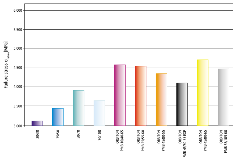
Figure 7.16. Results of comparative tests for the failure stress \sigma_{failure} for AC 16S with 10 bituminous binders manufactured by ORLEN Asphalt
