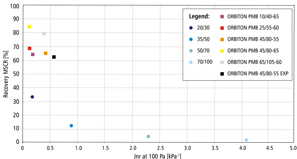
Figure 8.4. Presentation of bitumen results on the MSCR chart: elastic deformation R as a function of J_{nr} at the load of 0.1 kPa, at 64°C (the smaller J_{nr} the greater rutting resistance, the greater recovery, the more elastic the binder)
