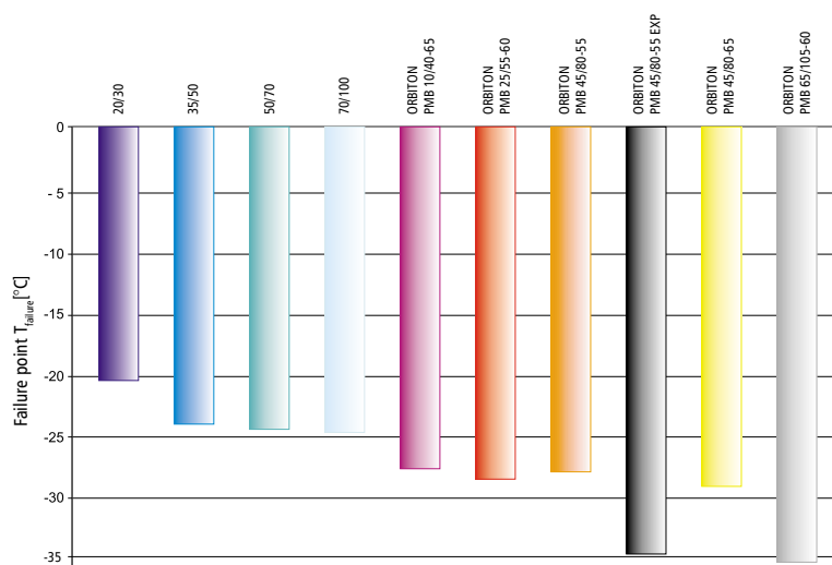
Figure 7.15. Results of comparative tests for the failure point T_{failure} for AC 16S with 10 bituminous binders manufactured by ORLEN Asphalt
