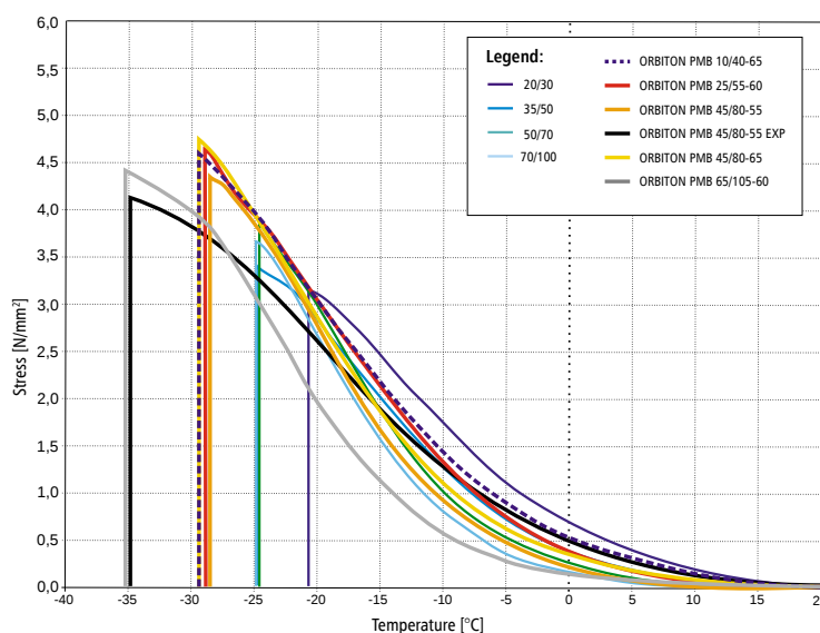
Figure 7.17. Results of comparative tests for the difference in the tension stress in the course of the TSRST depending on temperature \sigma_{cry} (T) for AC 16S with 10 bituminous binders manufactured by ORLEN Asphalt
