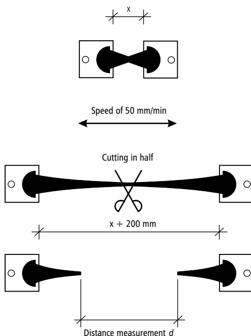
Figure 2.26. Elastic recovery test principle
