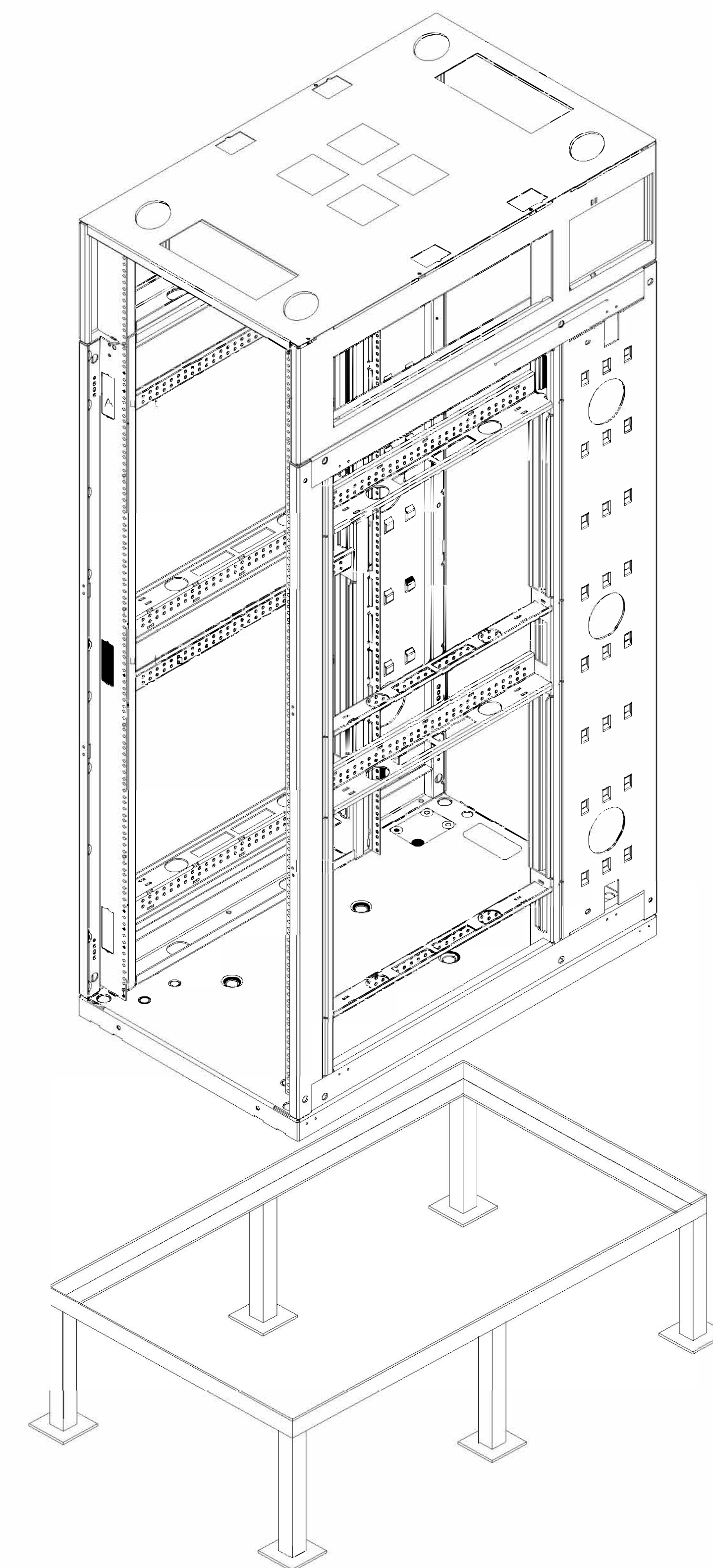
Isometric View
