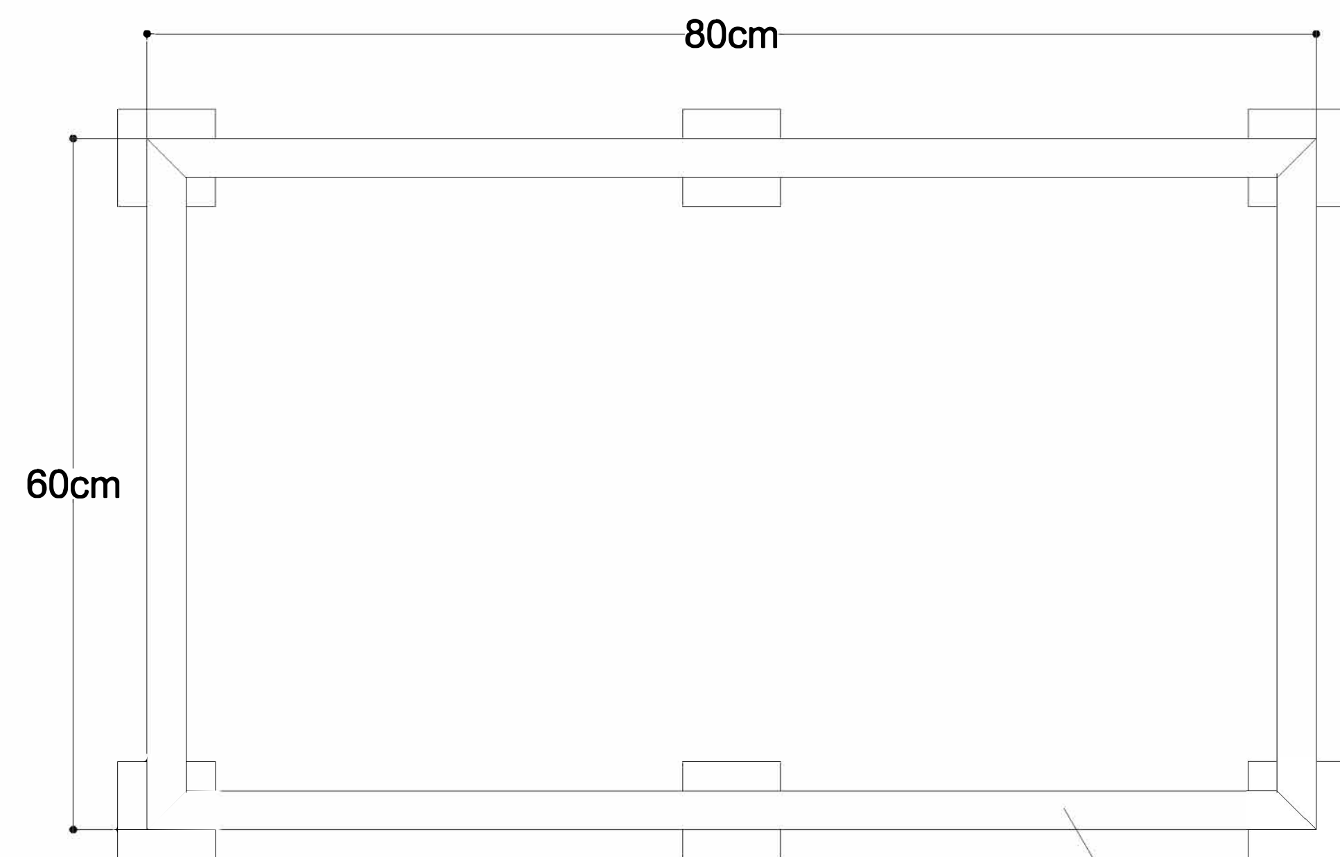
Top View
